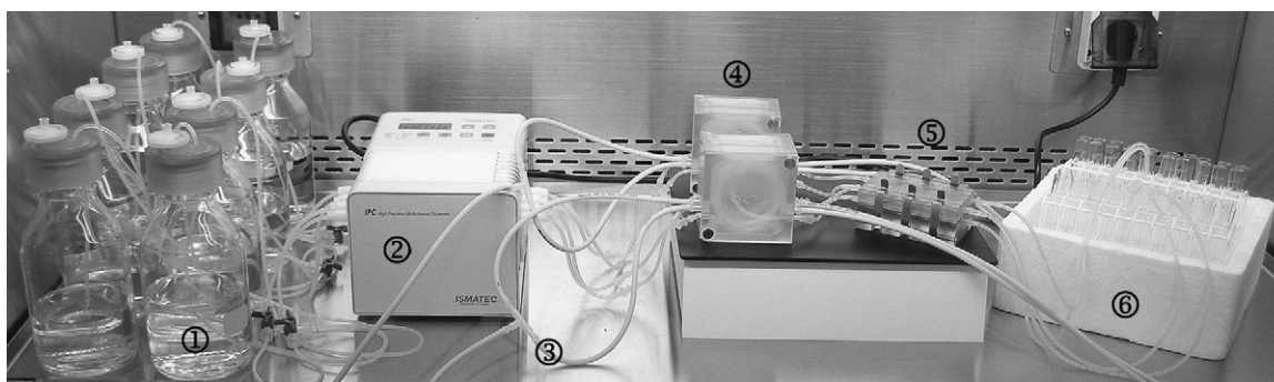
Fig. 1. Components of perfusion culture set. 1 – storage medium bottles; 2 – peristaltic pump; 3 – connecting fittings between air pump or gas bottle and gas exchange module; 4 – two gas exchange modules; 5 – gradient culture container; 6 – sampling vials. Perfusion culture set 1 used in Experiments 1 and 2 consists of components 1, 2, 5 and 6. Perfusion culture set 2 used in Experiment 3 consists of all components with one gas exchange module. Perfusion culture set 3 used in Experiment 4 consists of all components with double gas exchange module.
