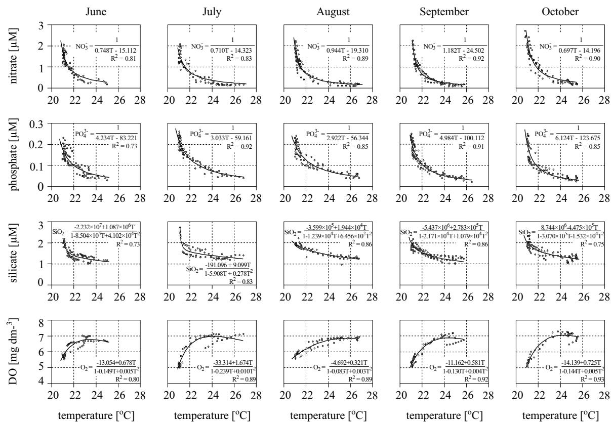
Fig. 5. Relationships between seawater temperature [ ^{\circ}\text{C} ] versus nitrate [ \mu\text{M} ], phosphate [ \mu\text{M} ], silicate [ \mu\text{M} ] and oxygen [ \text{mg dm}^{-3} ] in the offshore water of the northern Gulf of Aqaba during summer months (June–October). Every month represents the average of the five years: 1998, 2000–2003
