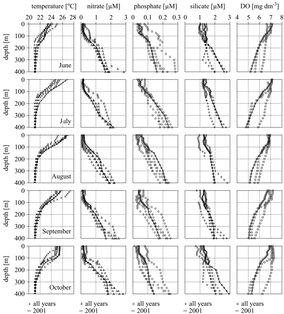
Fig. 3. Nitrate [ \mu\text{M} ], phosphate [ \mu\text{M} ], silicate [ \mu\text{M} ] and oxygen [ \text{mg dm}^{-3} ] profiles in the offshore water of the northern Gulf of Aqaba during the summer months (June–October) of every year observed (1998, 2000–2003)
