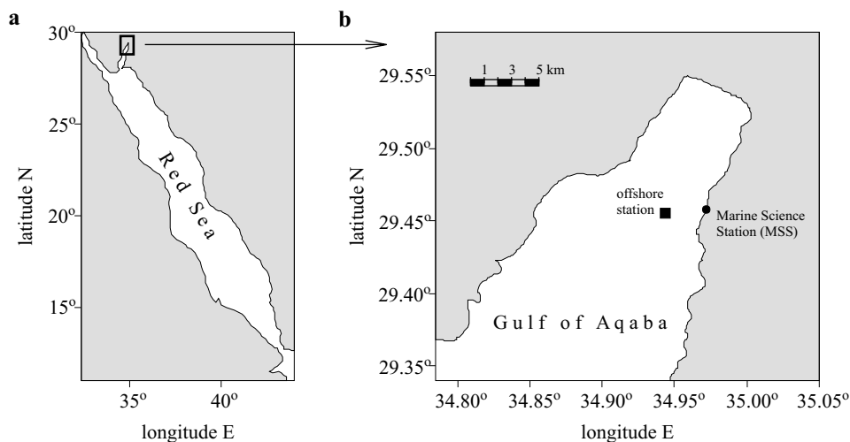
Fig. 1. Study site (a), offshore site for temperature [ ^{\circ}\text{C} ], nutrients [ \mu\text{M} ] and oxygen [ \text{mg dm}^{-3} ] sampling (b)
