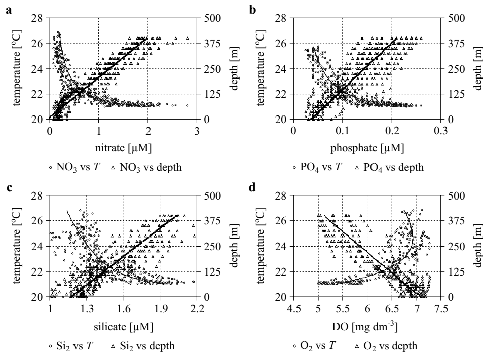
Fig. 4. Nutrients [ \mu\text{M} ] and dissolved oxygen [ \text{mg dm}^{-3} ] relationships with temperature [ ^{\circ}\text{C} ] and depth [m] in the offshore water of the northern Gulf of Aqaba during the summer months (June–October) of every year observed (1998, 2000–2003)
