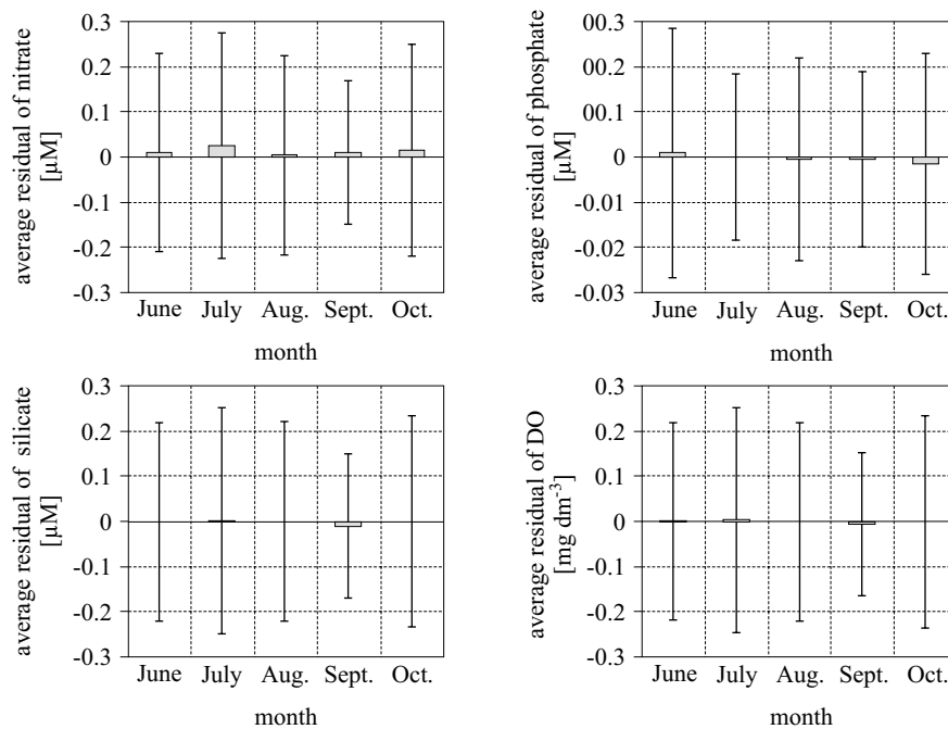
Fig. 6. The average of anomalies values between the real observations and the best fit relationship of nitrate [ \mu\text{M} ], phosphate [ \mu\text{M} ], silicate [ \mu\text{M} ] and oxygen [ \text{mg dm}^{-3} ] during the summer months (June–October) of every year observed (1998, 2000–2003)
