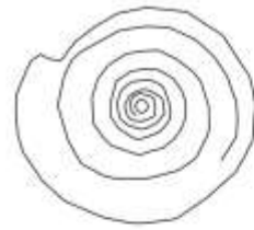
Cornuspira involvens
