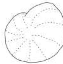
Elphidium excavatum
